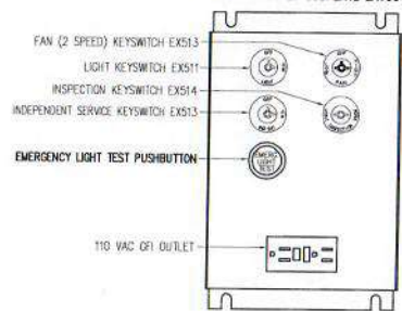
SERVICE CABINET SUBPLATE LAYOUT
