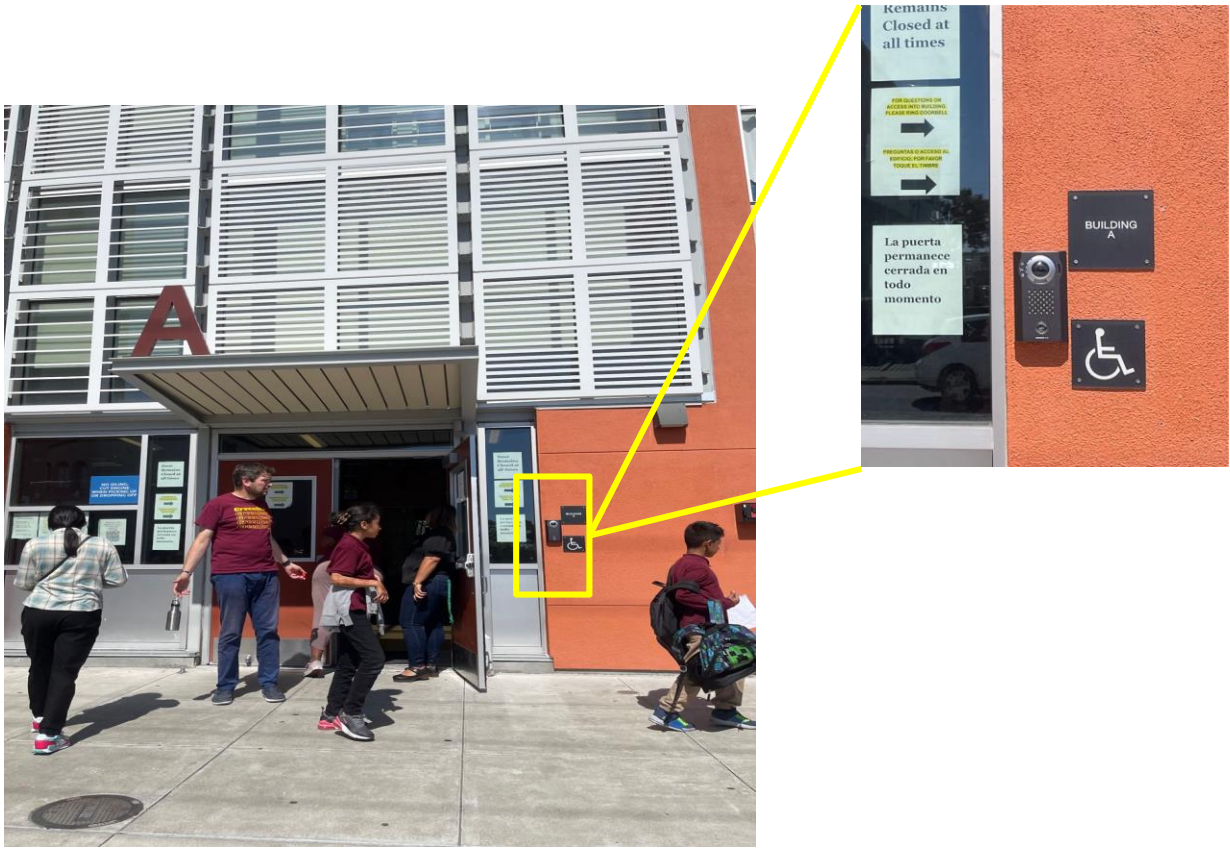
Wall-mounted Aiphone IX-DV door station
