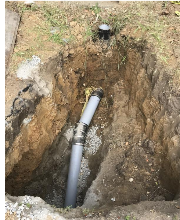
After - Replaced with High Density Polyethylene piping
