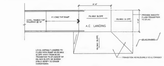
6 A.C. LANDING AT PRE-MANUFACTURED RAMP SCALE: 3/8\"/>
