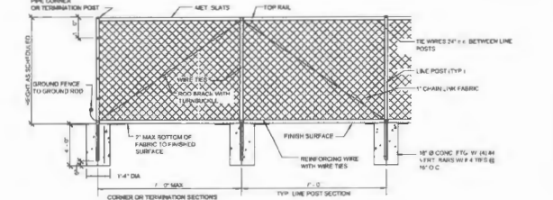
17 CHAIN LINK FENCE/FOOTING SCALE: 3/8\"/>
