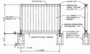
7 WOOD FENCE ELEVATION SCALE: 3/8\"/>
