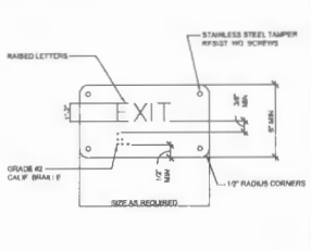
21 TACTILE EXIT SIGN SCALE: 3/8\"/>
