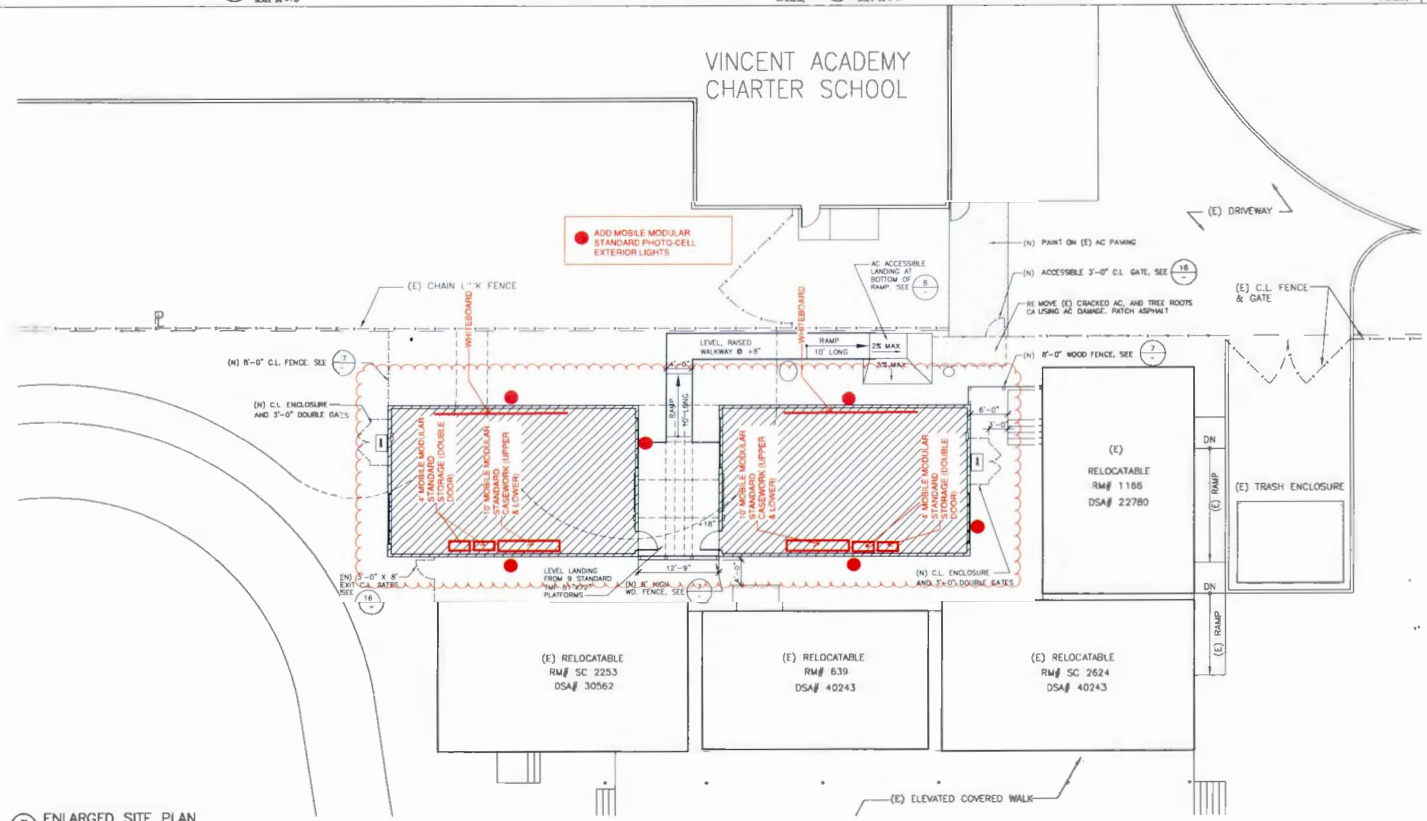
5 ENLARGED SITE PLAN SCALE: 1/8\"/>
