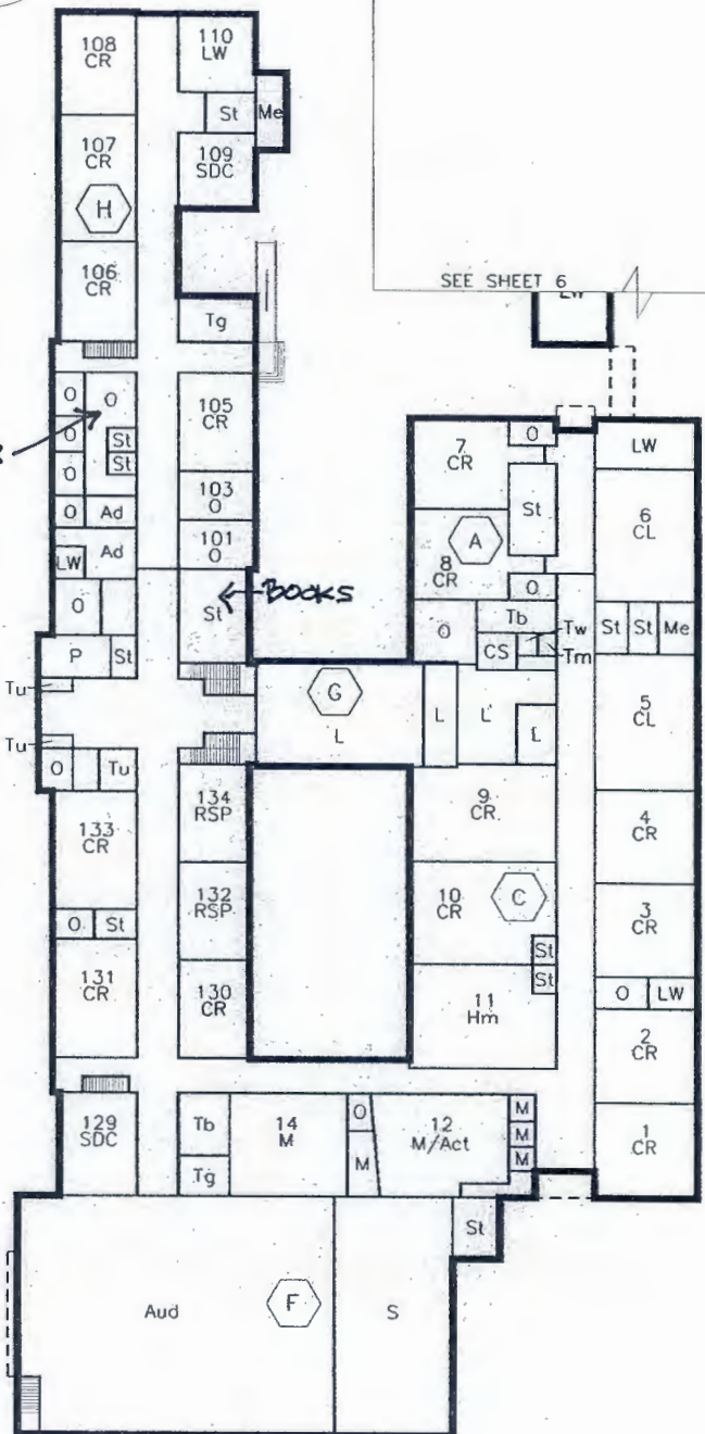
1 FIRST FLOOR PLAN 1" = 60'-0"
