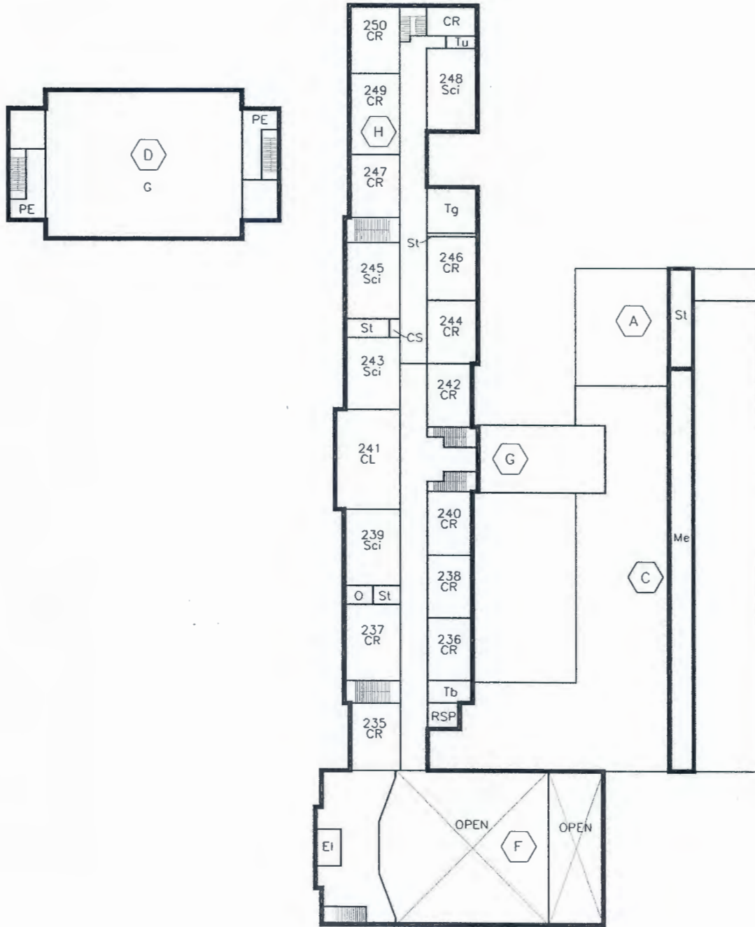
1 SECOND FLOOR PLAN 1" = 60'-0"
