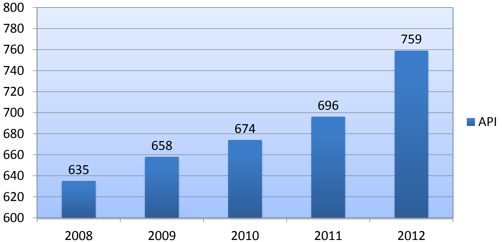
API Scores
